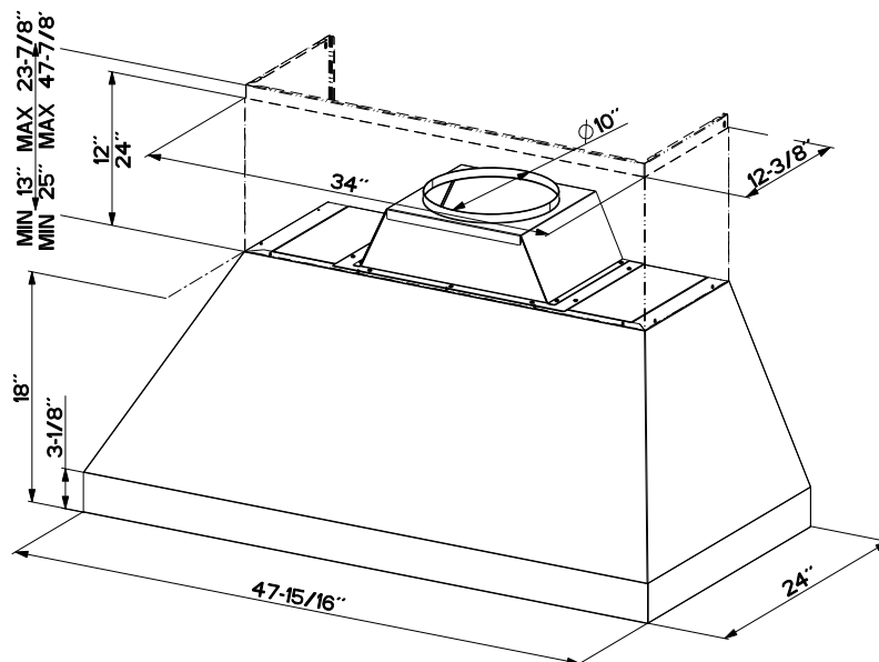
48" FRONT VIEW (SHOWN WITH CHIMNEY KIT)
