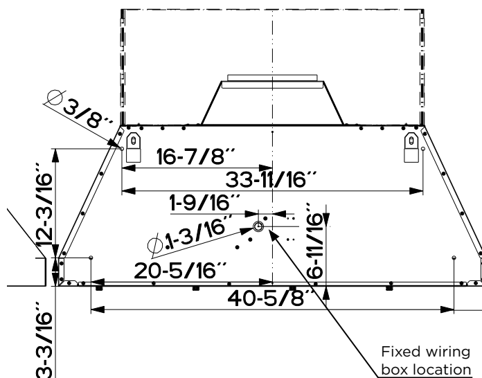
48" REAR VIEW (SHOWN WITH CHIMNEY KIT)
