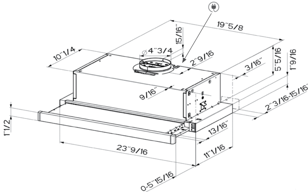
24" FRONT VIEW
