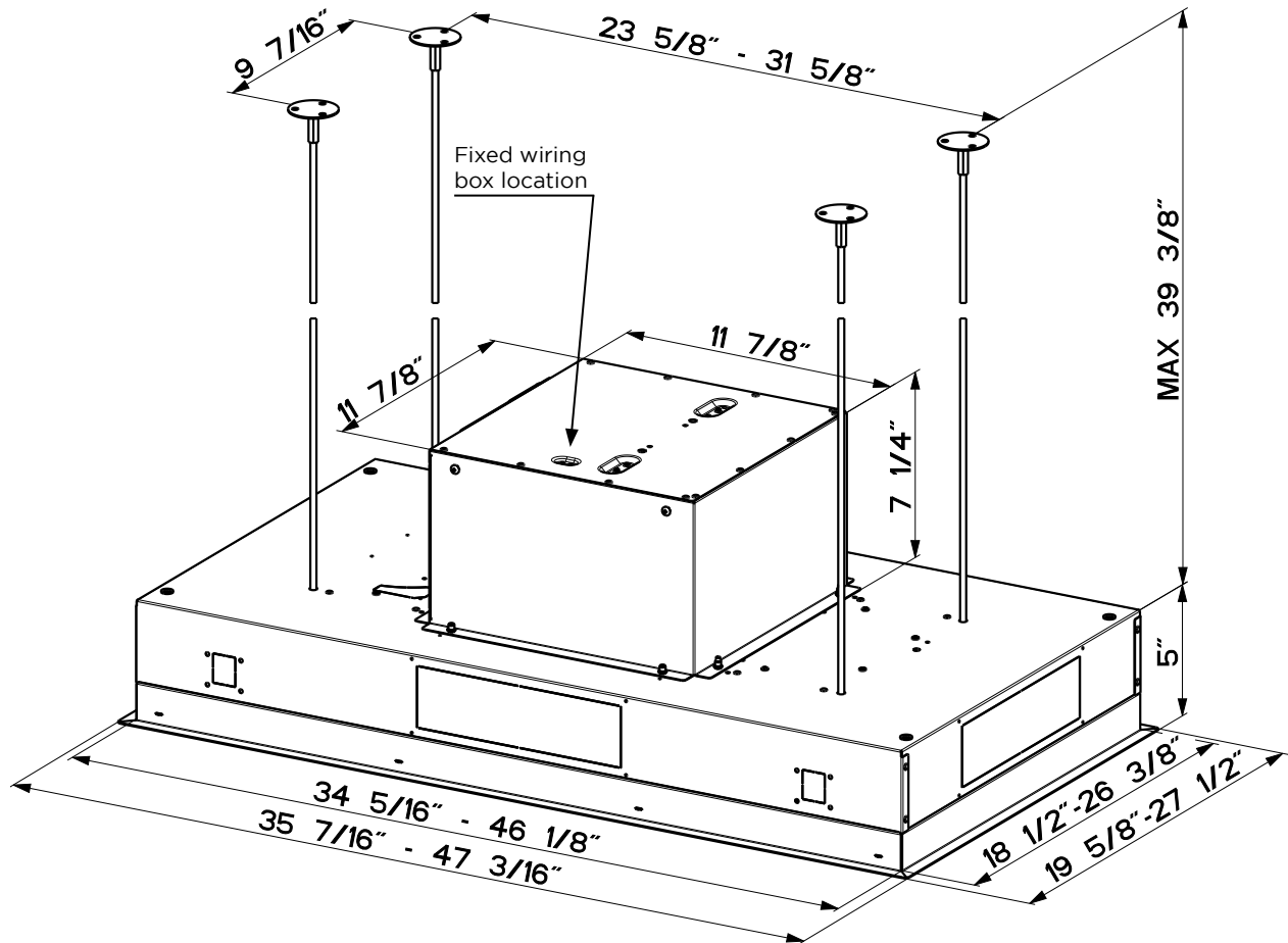
FRONT VIEW
