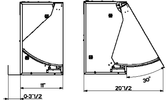
Side Views (Closed and Open)
